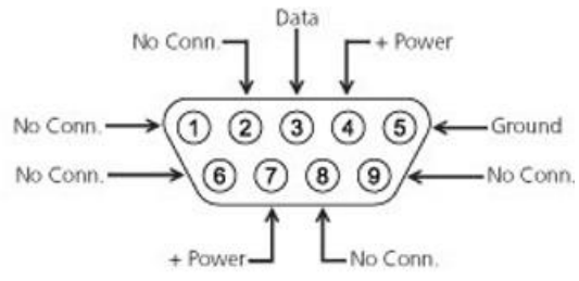
Fig. 2 9 Pin DB Connector
